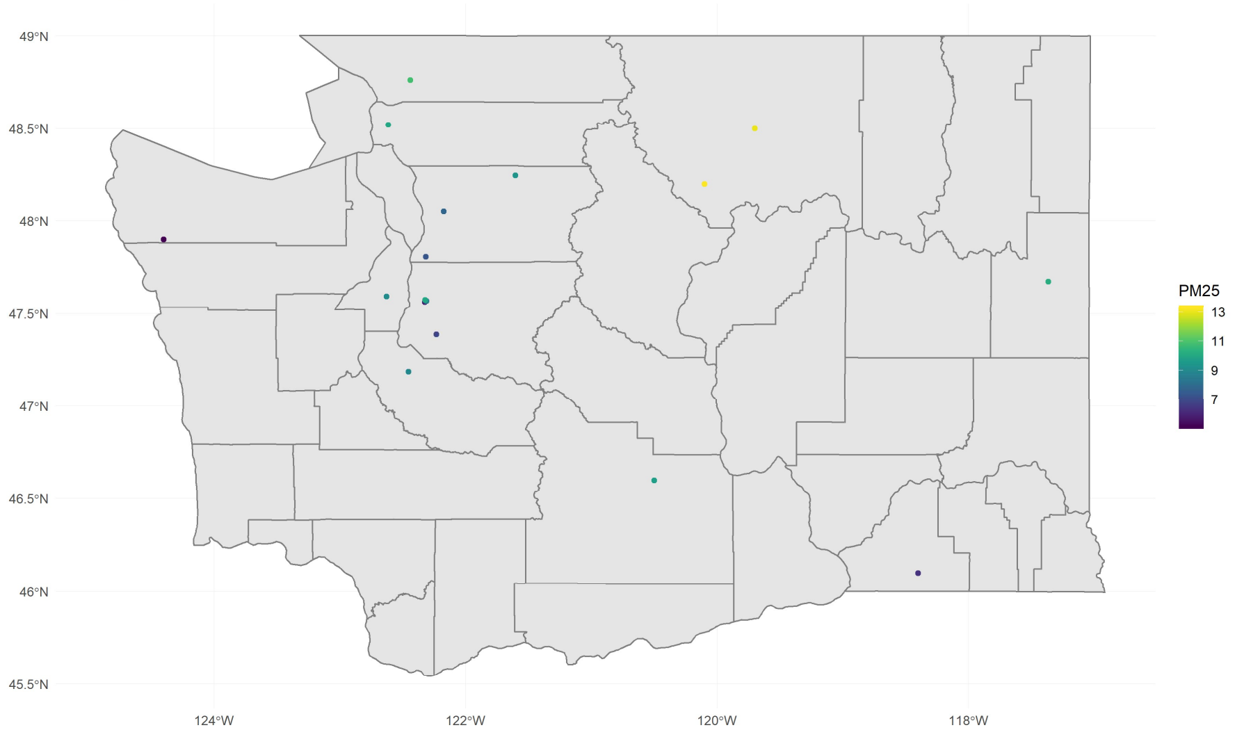
Washington PM25 - Mean Values
